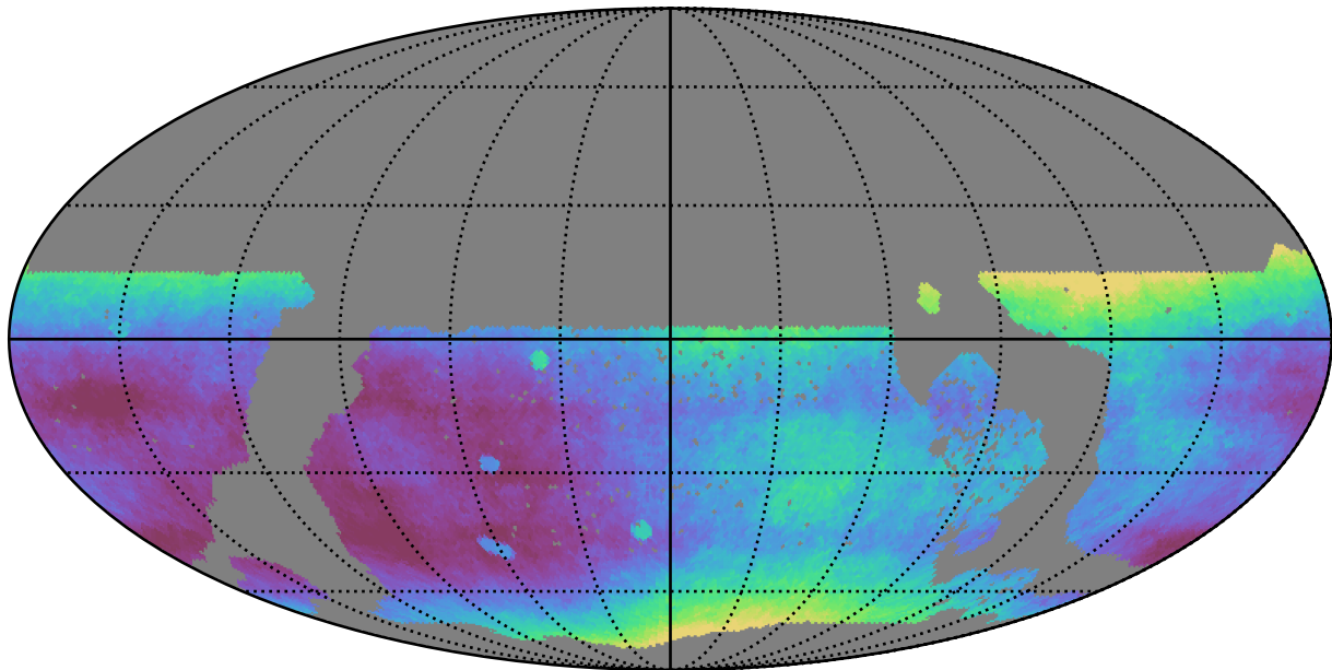
ddf_loaded_fl8_v3.4_10yrs WFD all bands: Median seeingEff
