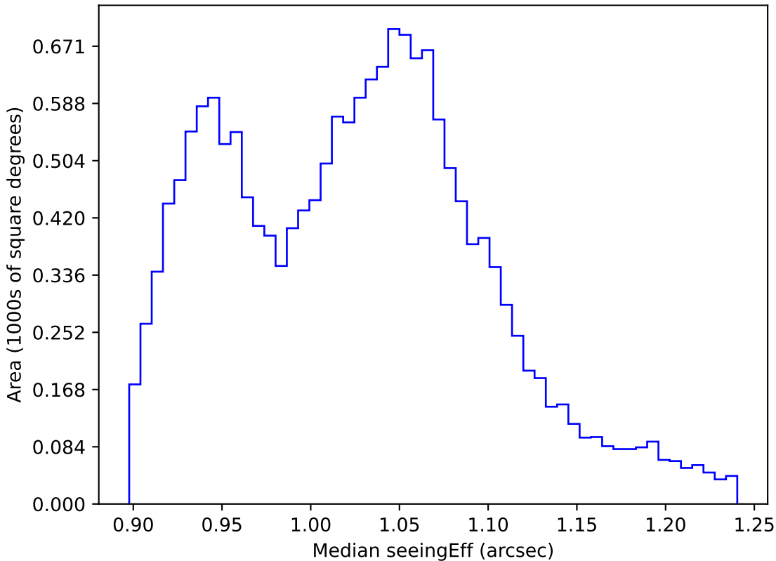
ddf_loaded_fl8_v3.4_10yrs WFD all bands: Median seeingEff
