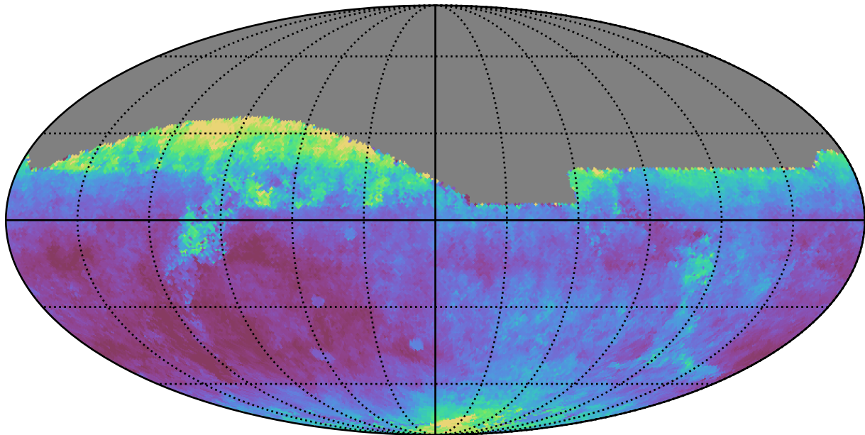
ddf_loaded_fl8_v3.4_10yrs All sky z band: Median seeingEff
