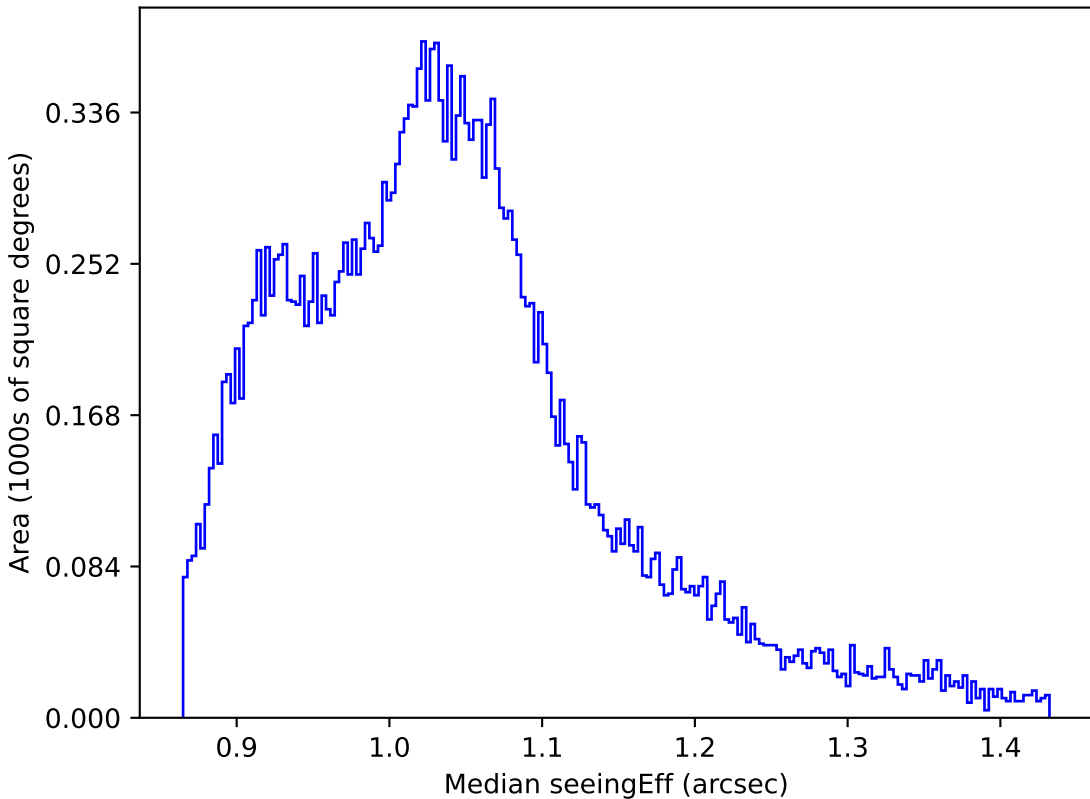
ddf_loaded_fl8_v3.4_10yrs All sky z band: Median seeingEff
