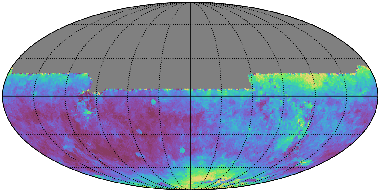
ddf_loaded_fl8_v3.4_10yrs All sky y band: Median seeingEff
