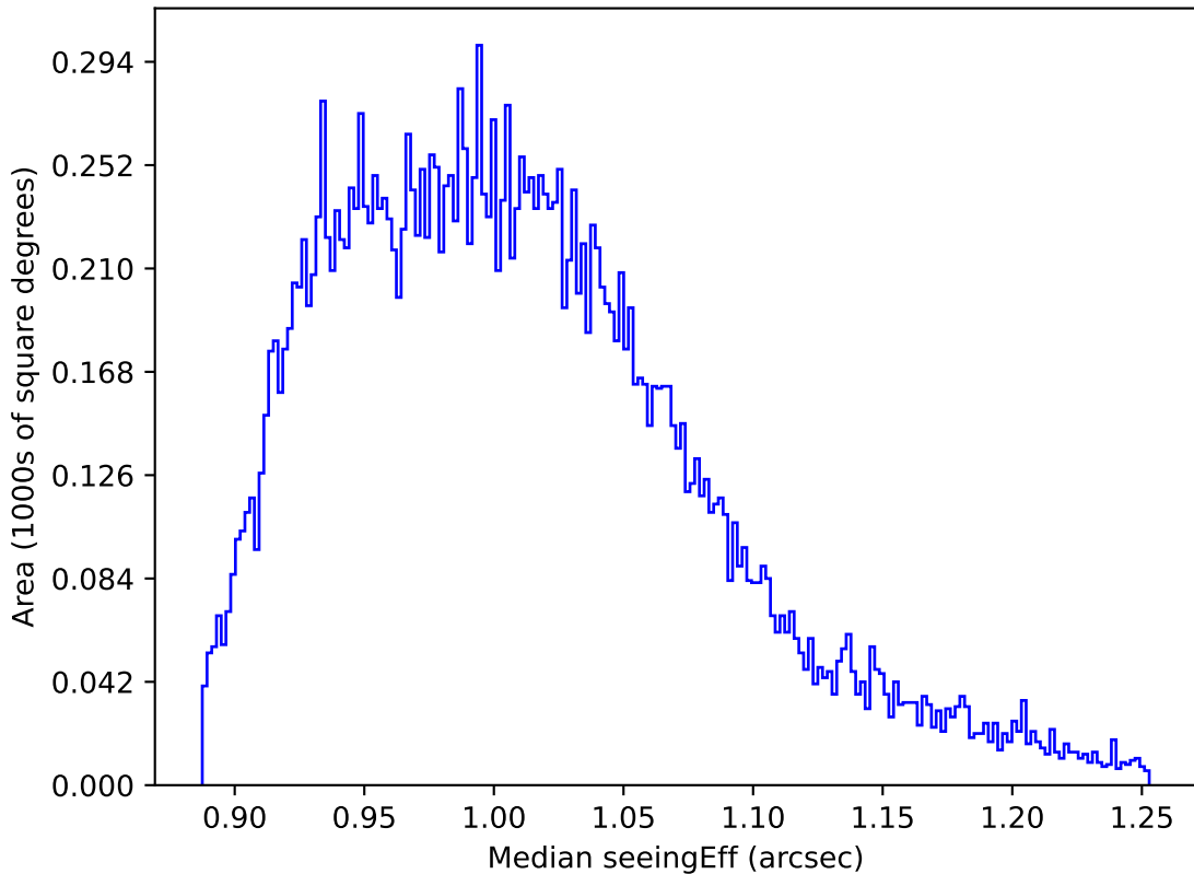
ddf_loaded_fl8_v3.4_10yrs All sky y band: Median seeingEff
