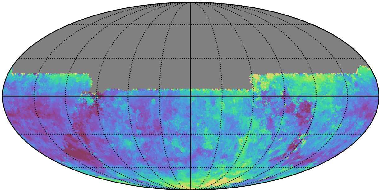
ddf_loaded_fl8_v3.4_10yrs All sky u band: Median seeingEff
