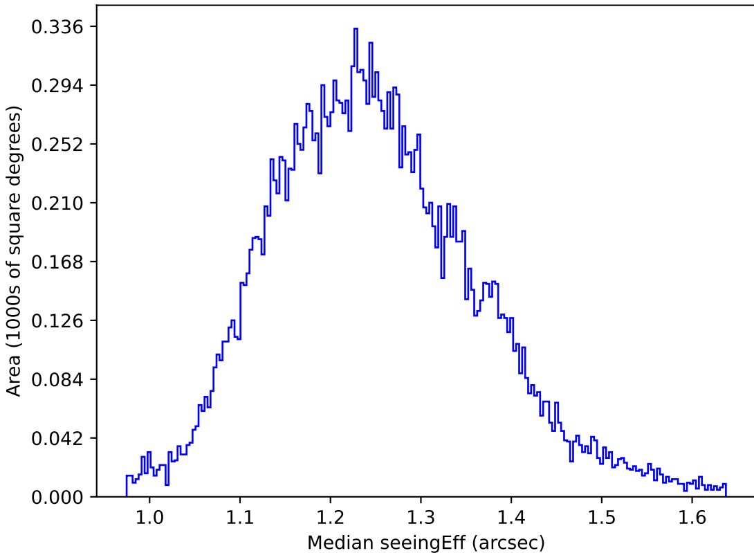
ddf_loaded_fl8_v3.4_10yrs All sky u band: Median seeingEff
