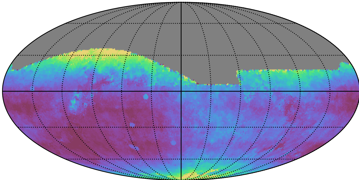
ddf_loaded_fl8_v3.4_10yrs All sky r band: Median seeingEff
