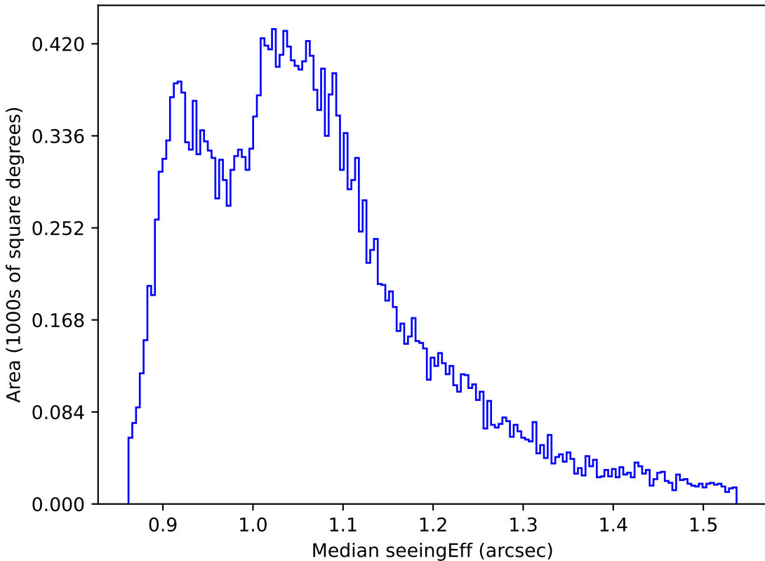
ddf_loaded_fl8_v3.4_10yrs All sky r band: Median seeingEff
