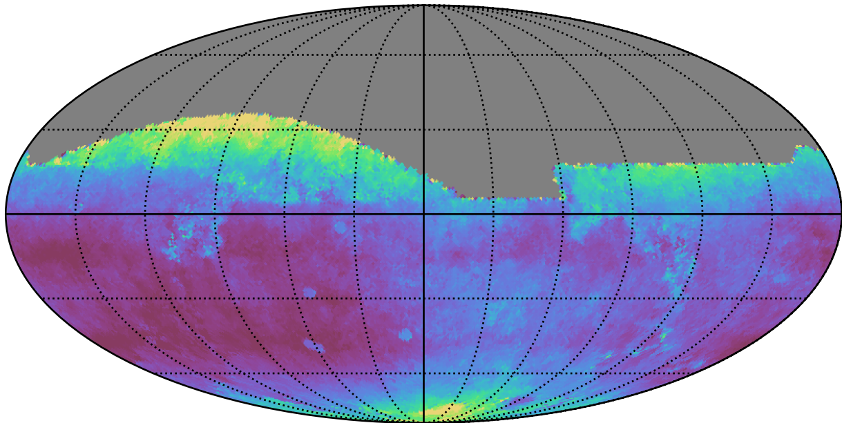
ddf_loaded_fl8_v3.4_10yrs All sky i band: Median seeingEff
