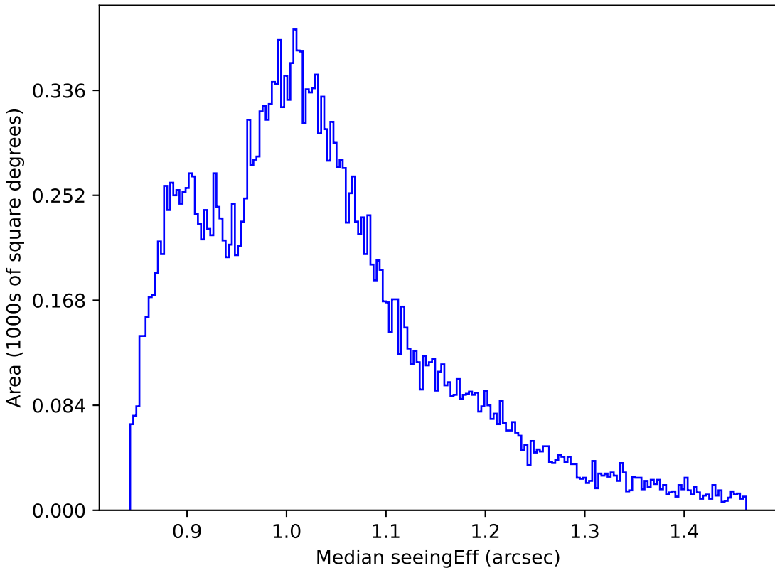
ddf_loaded_fl8_v3.4_10yrs All sky i band: Median seeingEff
