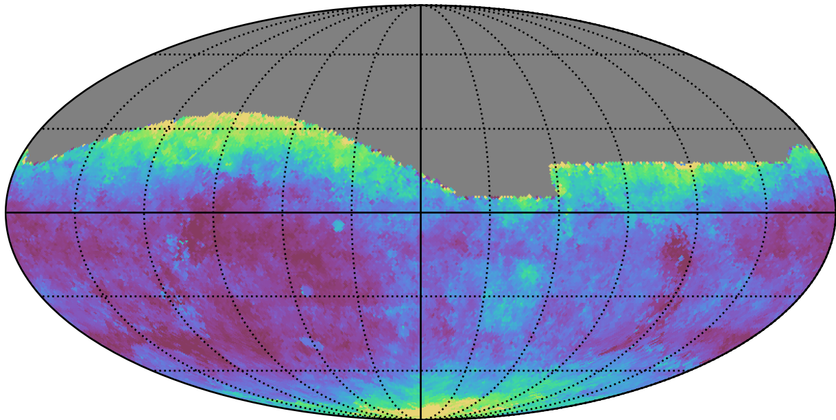
ddf_loaded_fl8_v3.4_10yrs All sky g band: Median seeingEff
