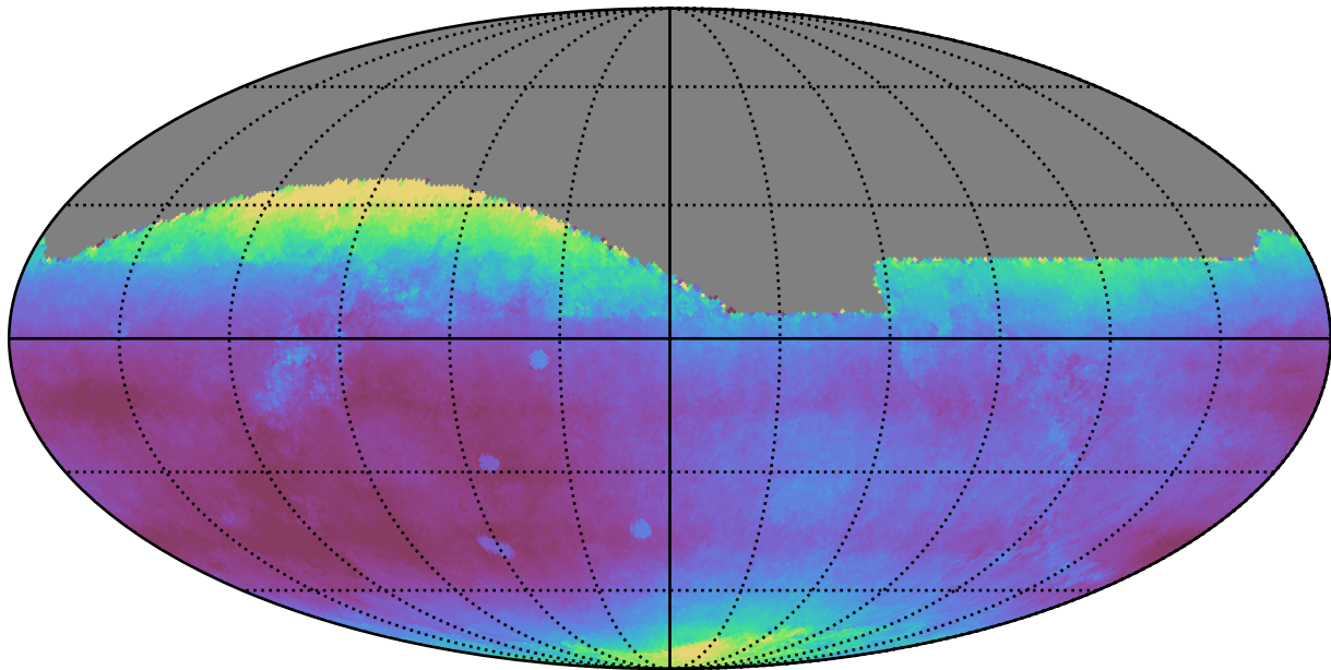
ddf_loaded_fl8_v3.4_10yrs All sky all bands: Median seeingEff
