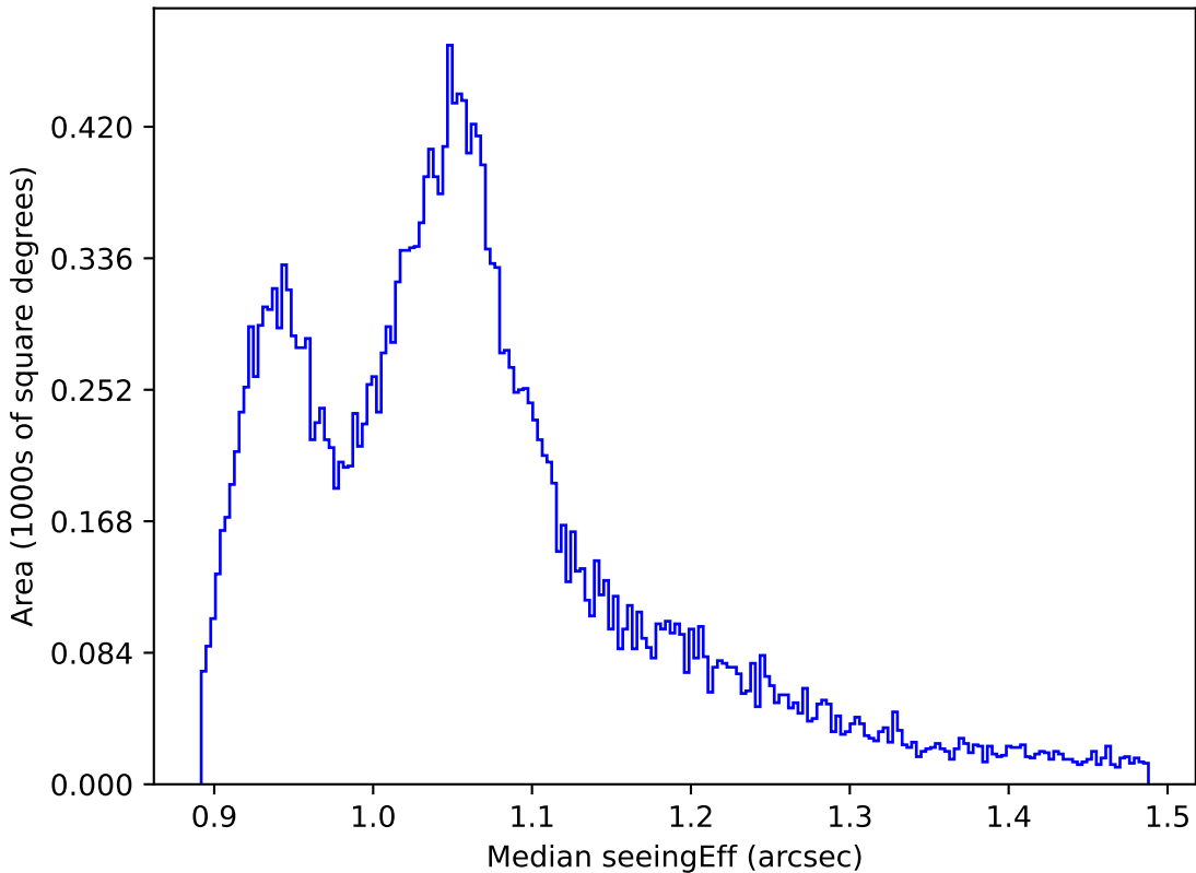
ddf_loaded_fl8_v3.4_10yrs All sky all bands: Median seeingEff
