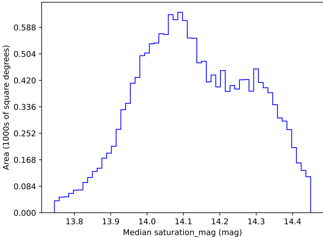
ddf_loaded_fl8_v3.4_10yrs WFD z band: Median saturation_mag
