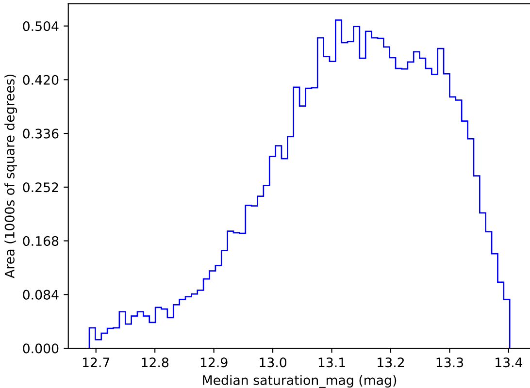
ddf_loaded_fl8_v3.4_10yrs WFD y band: Median saturation_mag
