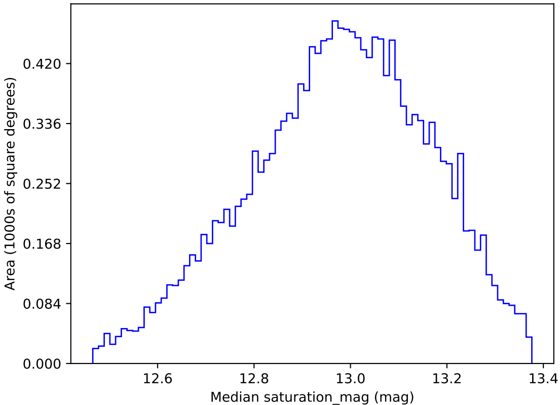
ddf_loaded_fl8_v3.4_10yrs WFD u band: Median saturation_mag
