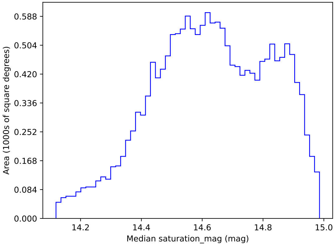
ddf_loaded_fl8_v3.4_10yrs WFD r band: Median saturation_mag
