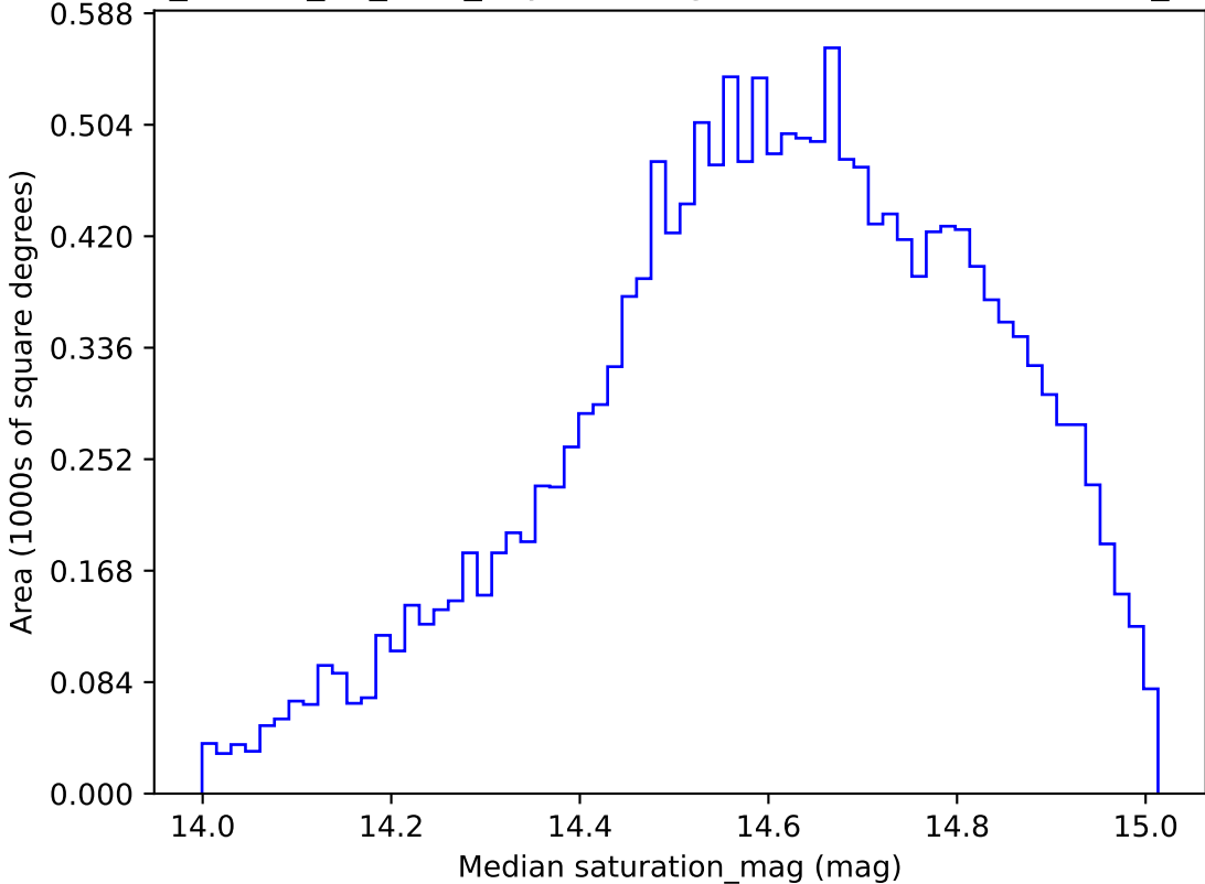
ddf_loaded_fl8_v3.4_10yrs WFD g band: Median saturation_mag
