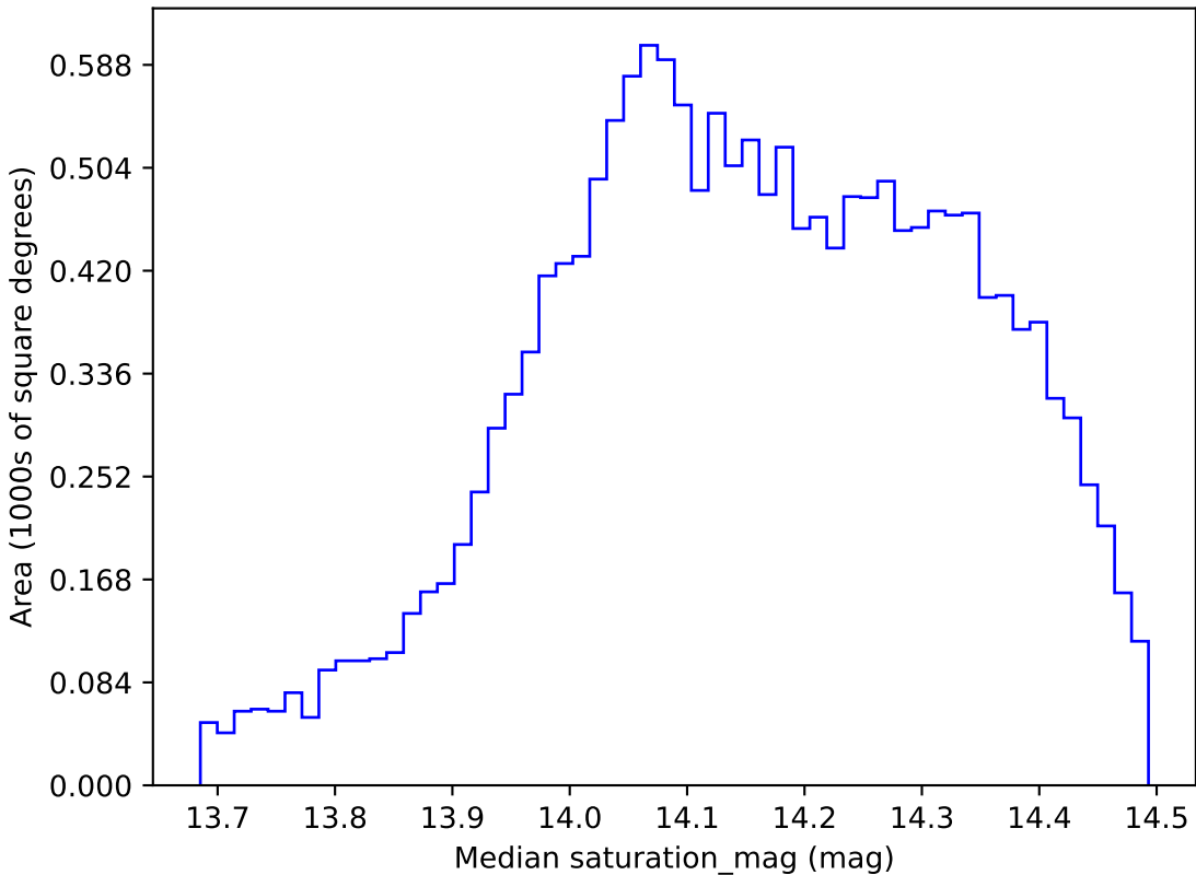
ddf_loaded_fl8_v3.4_10yrs WFD all bands: Median saturation_mag
