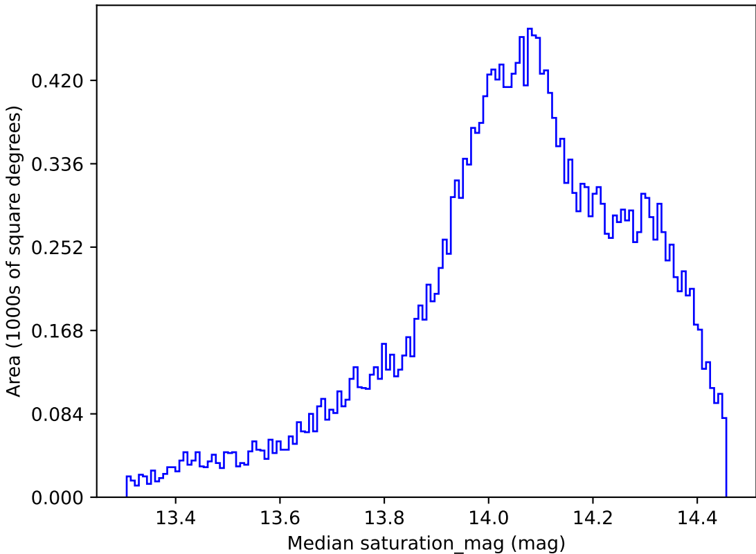
ddf_loaded_fl8_v3.4_10yrs All sky z band: Median saturation_mag
