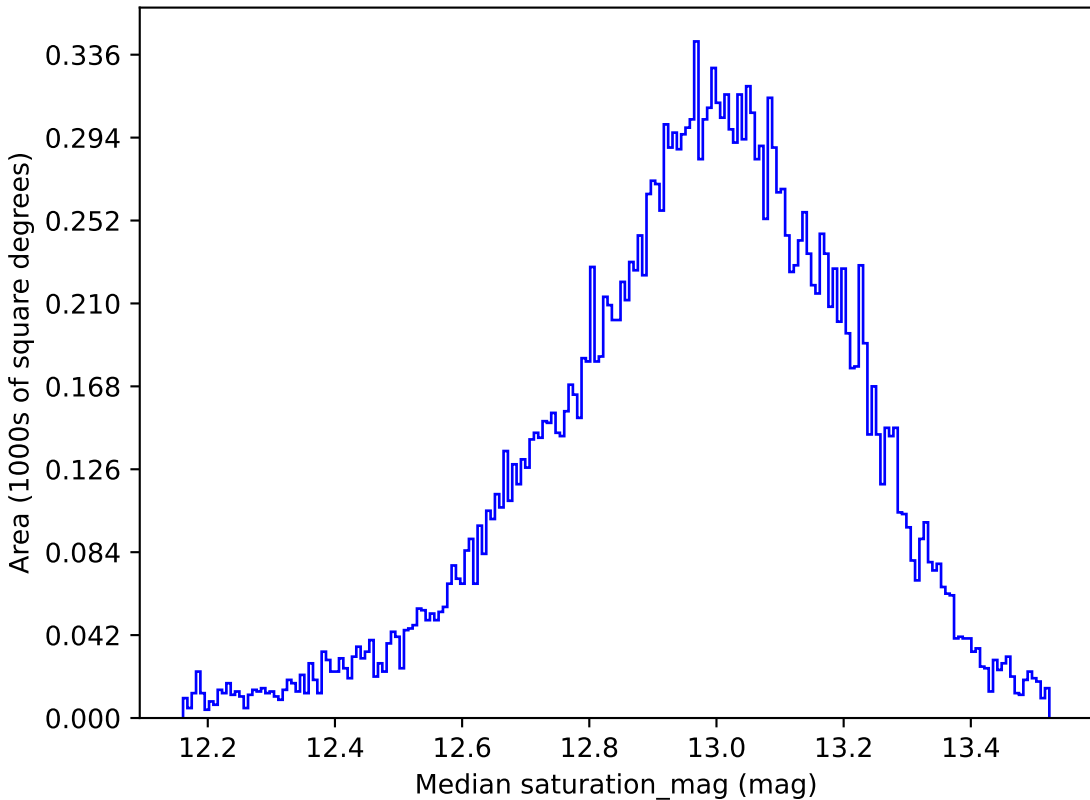
ddf_loaded_fl8_v3.4_10yrs All sky u band: Median saturation_mag
