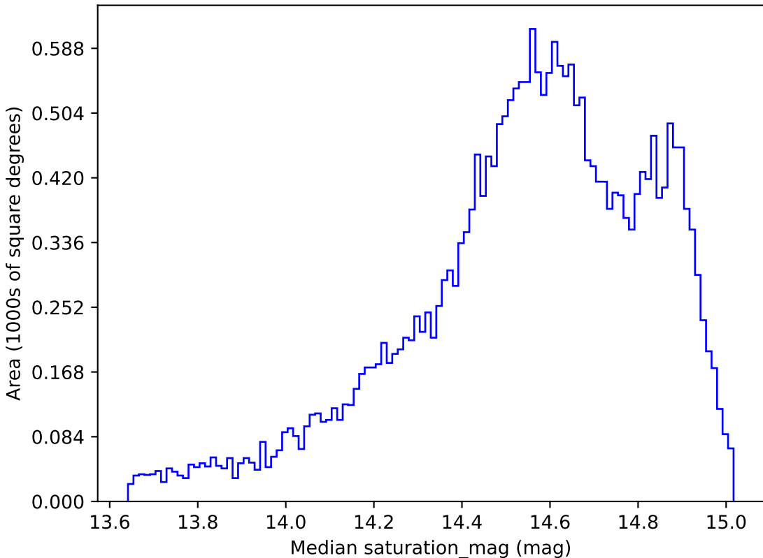
ddf_loaded_fl8_v3.4_10yrs All sky r band: Median saturation_mag
