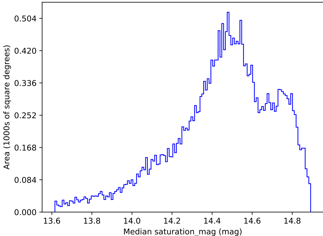
ddf_loaded_fl8_v3.4_10yrs All sky i band: Median saturation_mag
