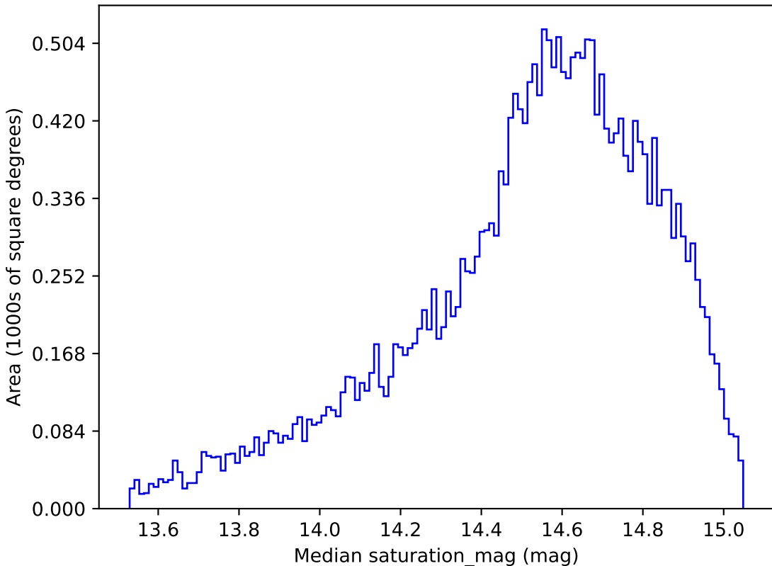
ddf_loaded_fl8_v3.4_10yrs All sky g band: Median saturation_mag
