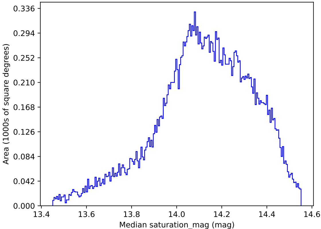
ddf_loaded_fl8_v3.4_10yrs All sky all bands: Median saturation_mag
