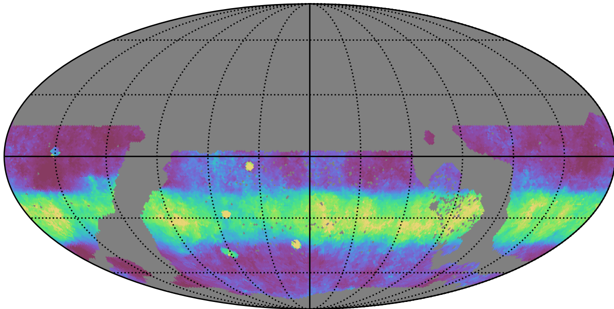
ddf_loaded_fl8_v3.4_10yrs WFD z band: Median normairmass
