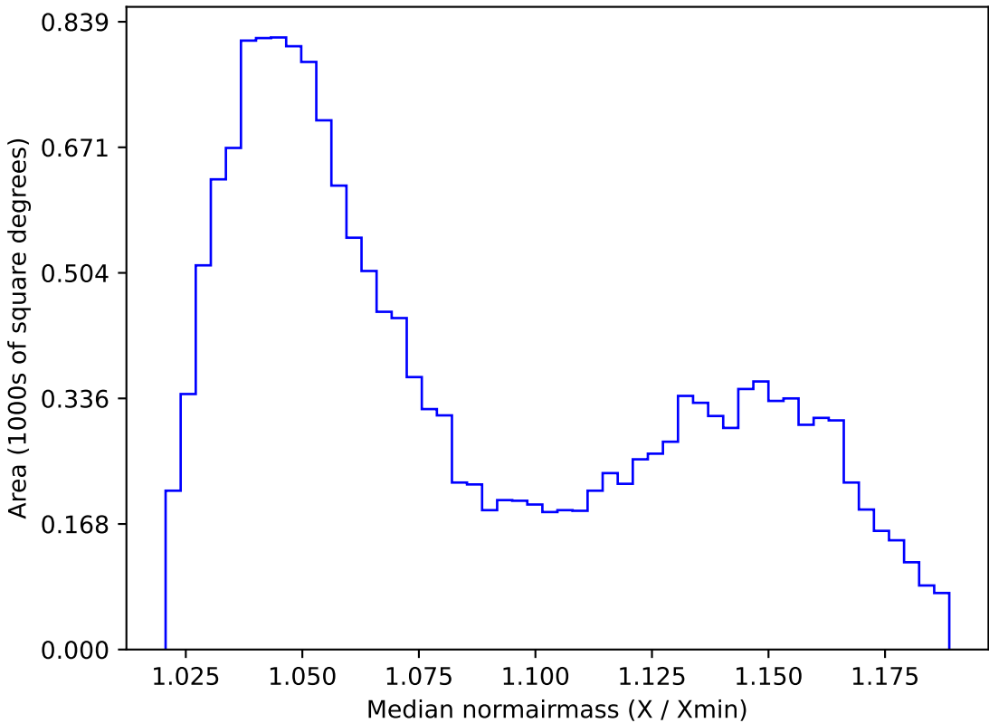
ddf_loaded_fl8_v3.4_10yrs WFD z band: Median normairmass
