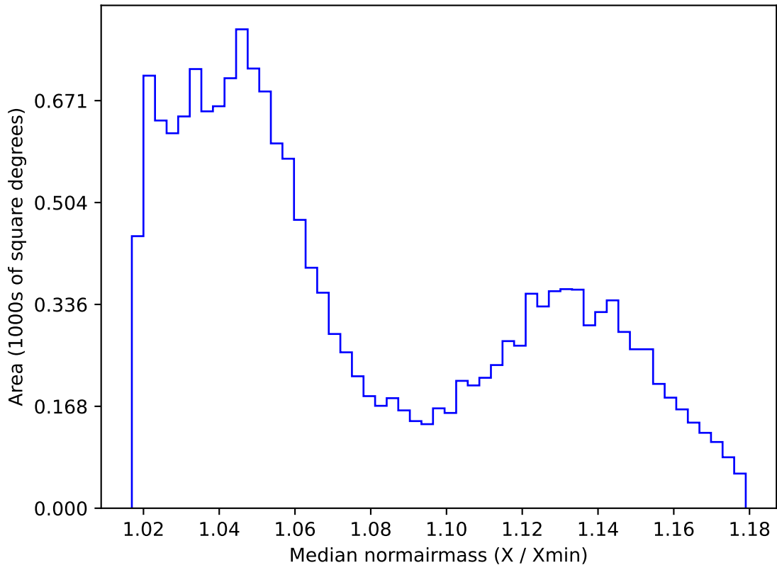
ddf_loaded_fl8_v3.4_10yrs WFD r band: Median normairmass
