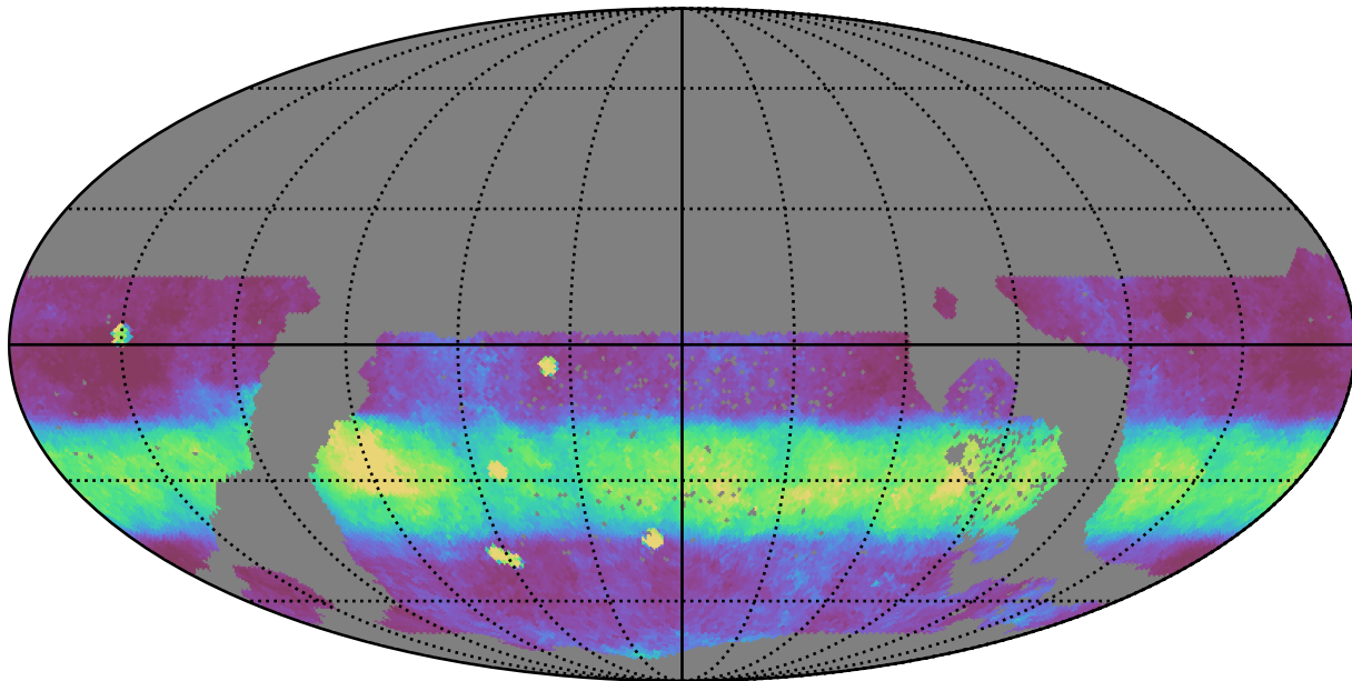
ddf_loaded_fl8_v3.4_10yrs WFD i band: Median normairmass
