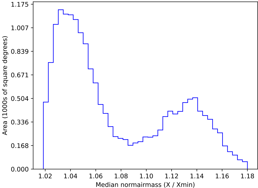
ddf_loaded_fl8_v3.4_10yrs WFD i band: Median normairmass
