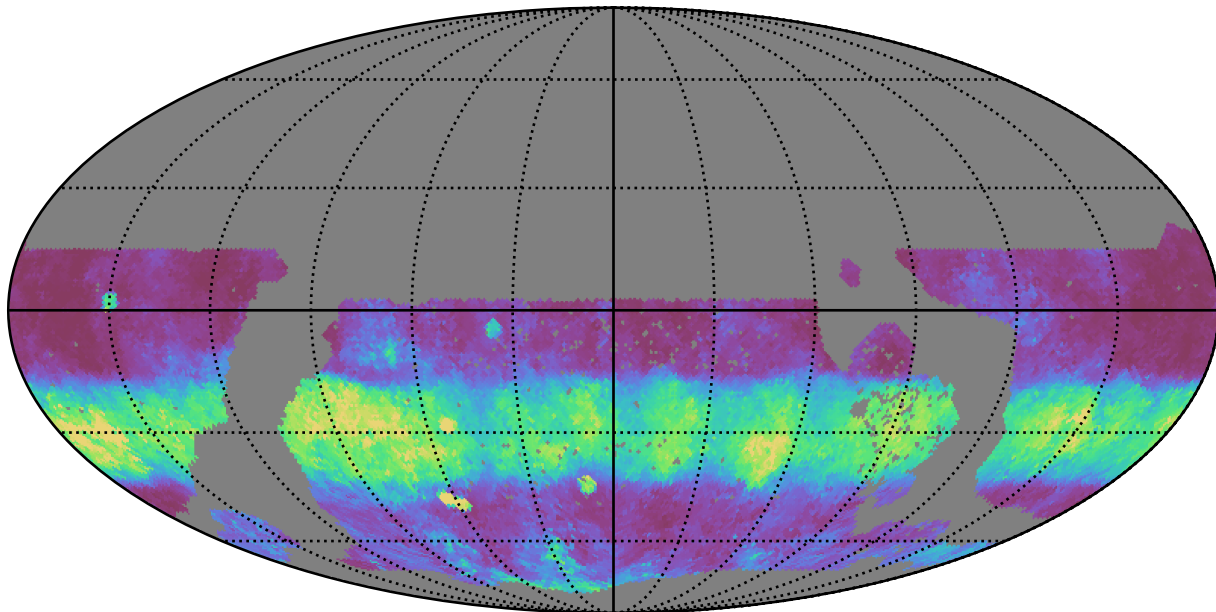
ddf_loaded_fl8_v3.4_10yrs WFD g band: Median normairmass
