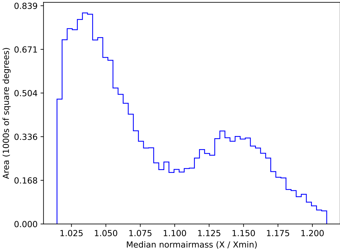
ddf_loaded_fl8_v3.4_10yrs WFD g band: Median normairmass
