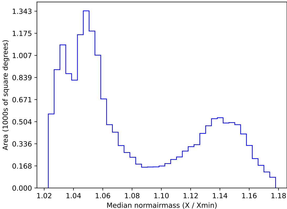
ddf_loaded_fl8_v3.4_10yrs WFD all bands: Median normairmass
