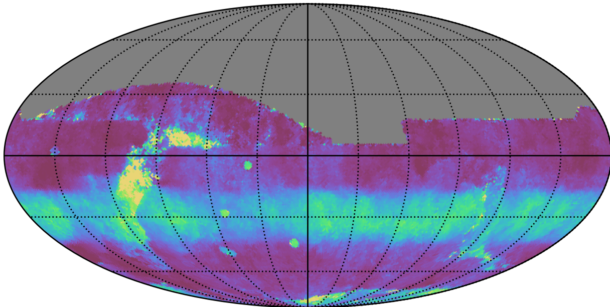
ddf_loaded_fl8_v3.4_10yrs All sky z band: Median normairmass
