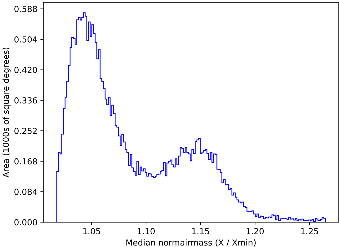
ddf_loaded_fl8_v3.4_10yrs All sky z band: Median normairmass
