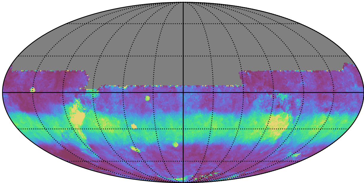
ddf_loaded_fl8_v3.4_10yrs All sky y band: Median normairmass
