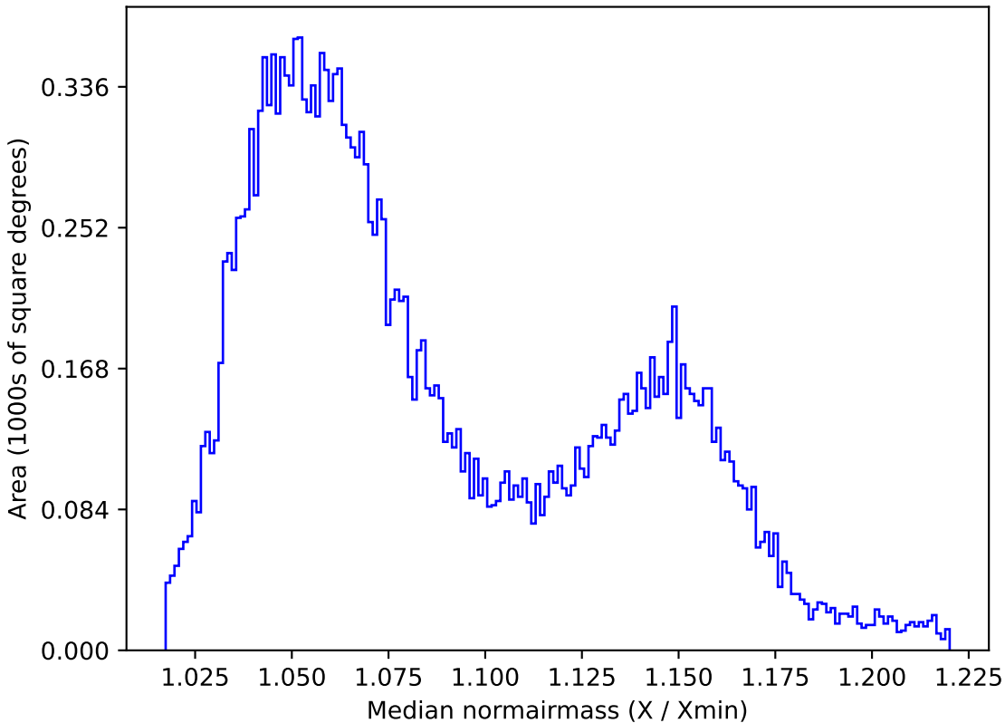
ddf_loaded_fl8_v3.4_10yrs All sky y band: Median normairmass
