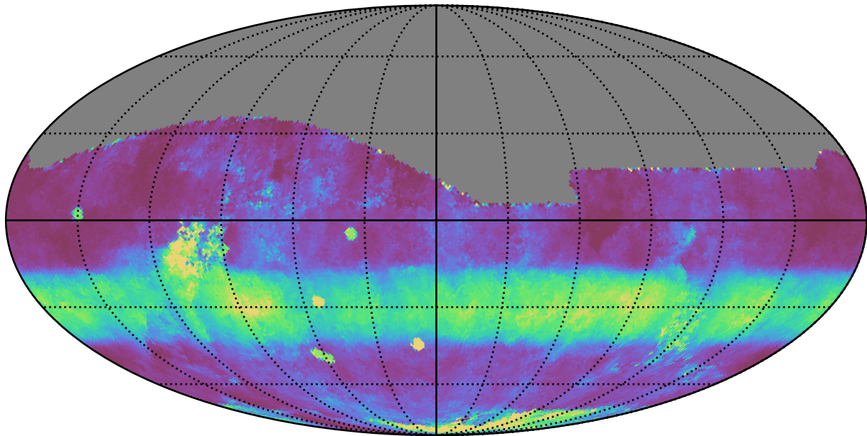
ddf_loaded_fl8_v3.4_10yrs All sky r band: Median normairmass
