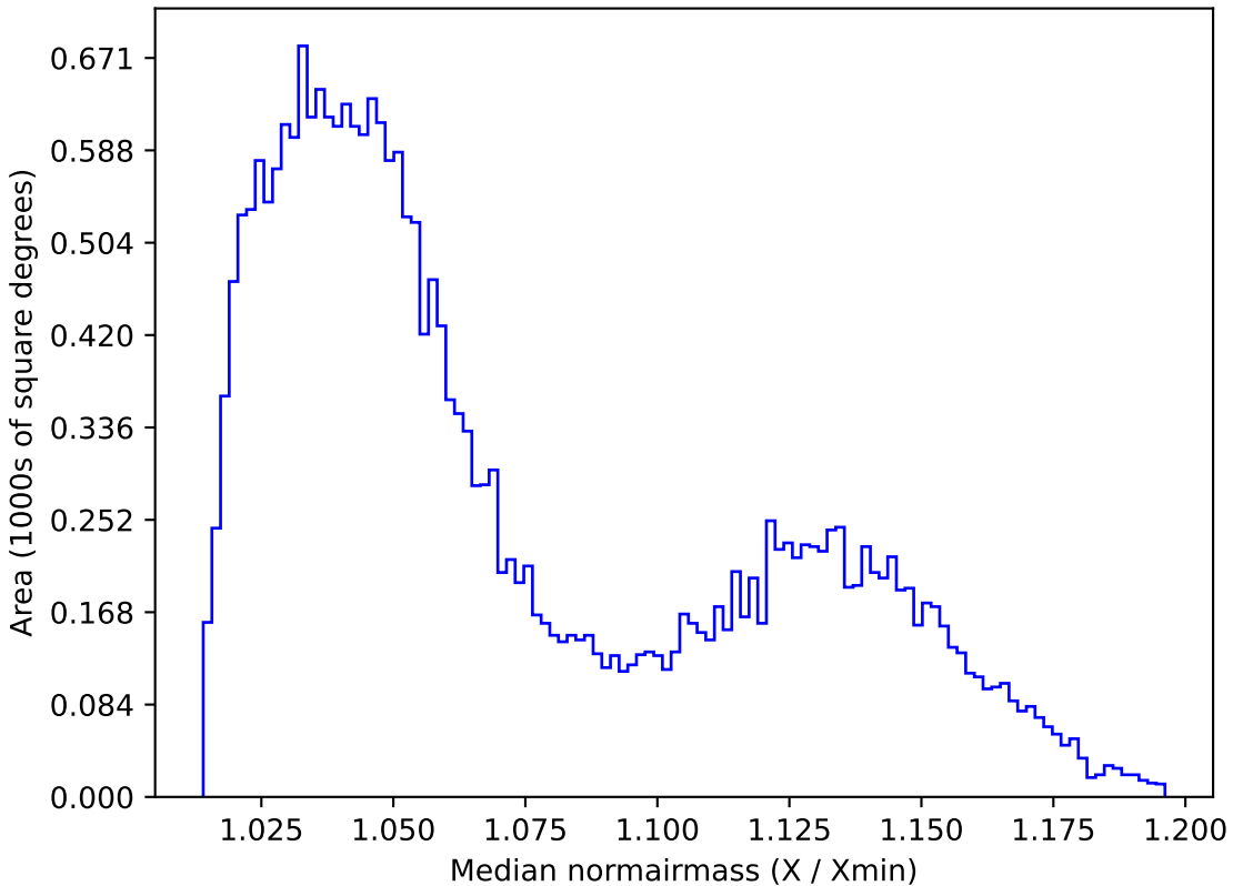
ddf_loaded_fl8_v3.4_10yrs All sky r band: Median normairmass
