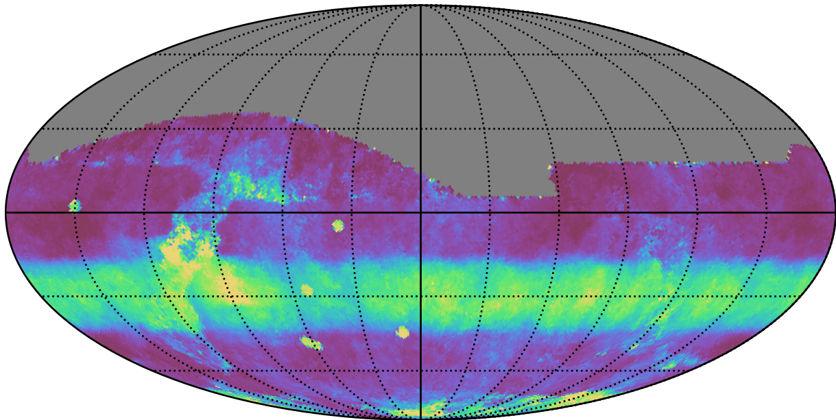
ddf_loaded_fl8_v3.4_10yrs All sky i band: Median normairmass
