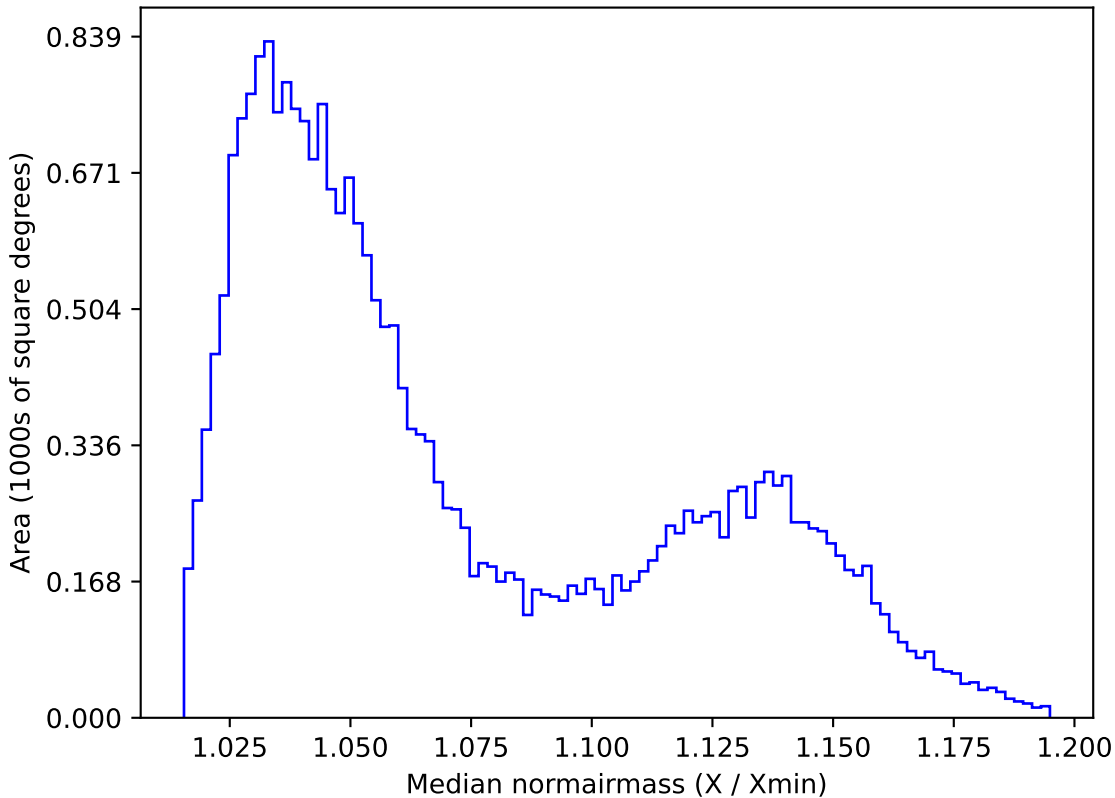
ddf_loaded_fl8_v3.4_10yrs All sky i band: Median normairmass
