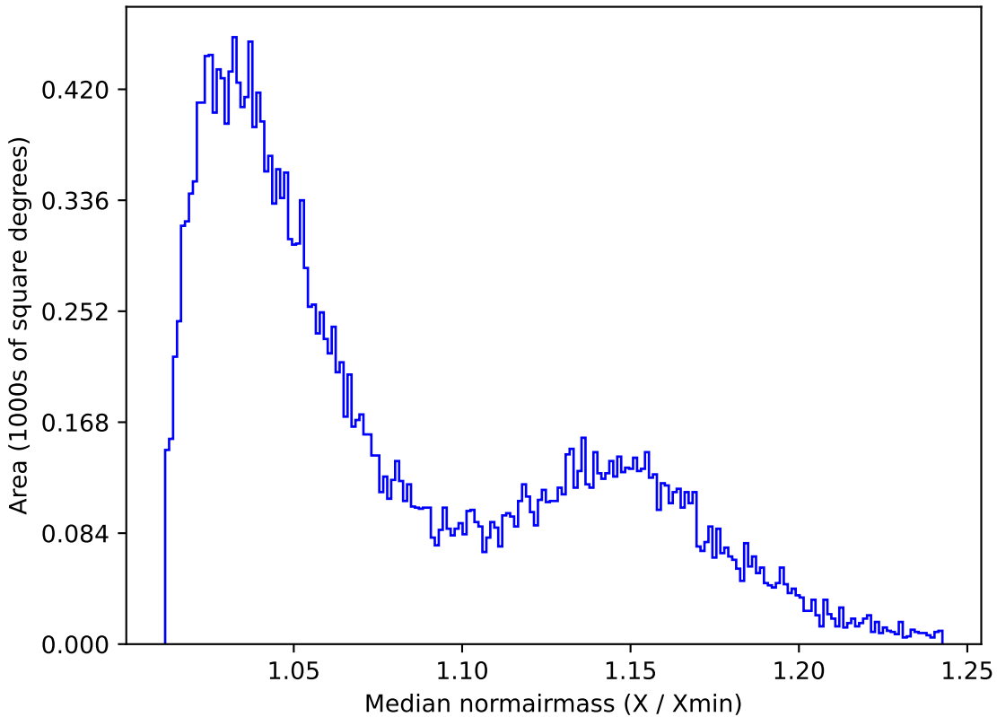
ddf_loaded_fl8_v3.4_10yrs All sky g band: Median normairmass
