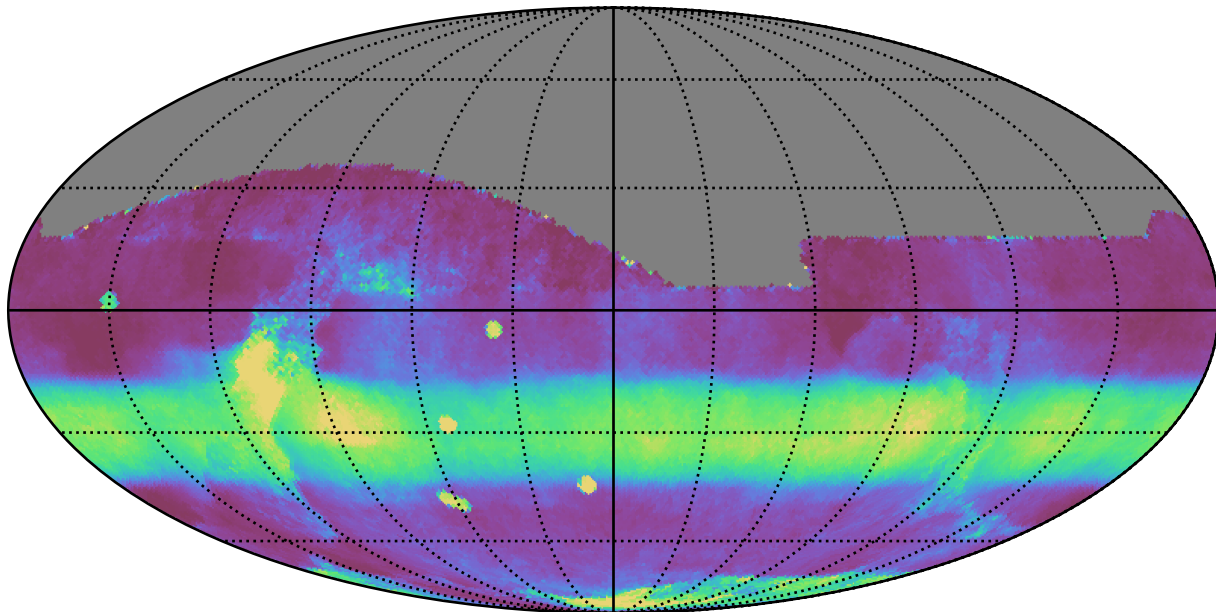
ddf_loaded_fl8_v3.4_10yrs All sky all bands: Median normairmass
