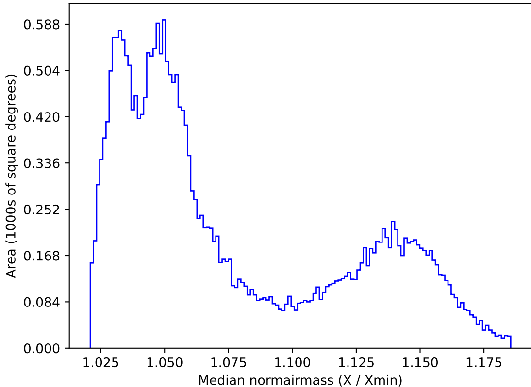
ddf_loaded_fl8_v3.4_10yrs All sky all bands: Median normairmass
