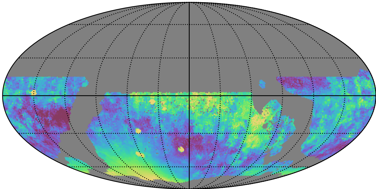
ddf_loaded_fl8_v3.4_10yrs WFD z band: Median moonDistance
