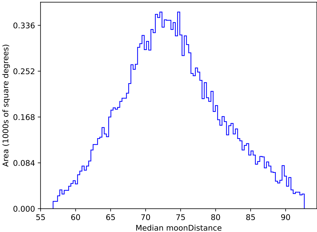
ddf_loaded_fl8_v3.4_10yrs WFD z band: Median moonDistance
