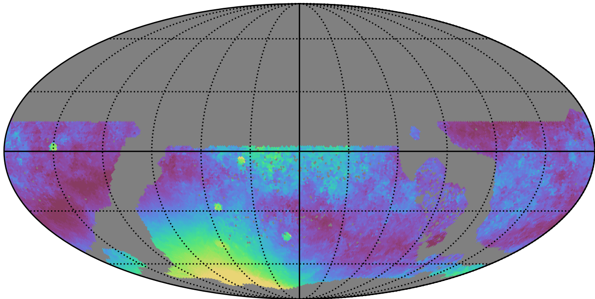
ddf_loaded_fl8_v3.4_10yrs WFD y band: Median moonDistance
