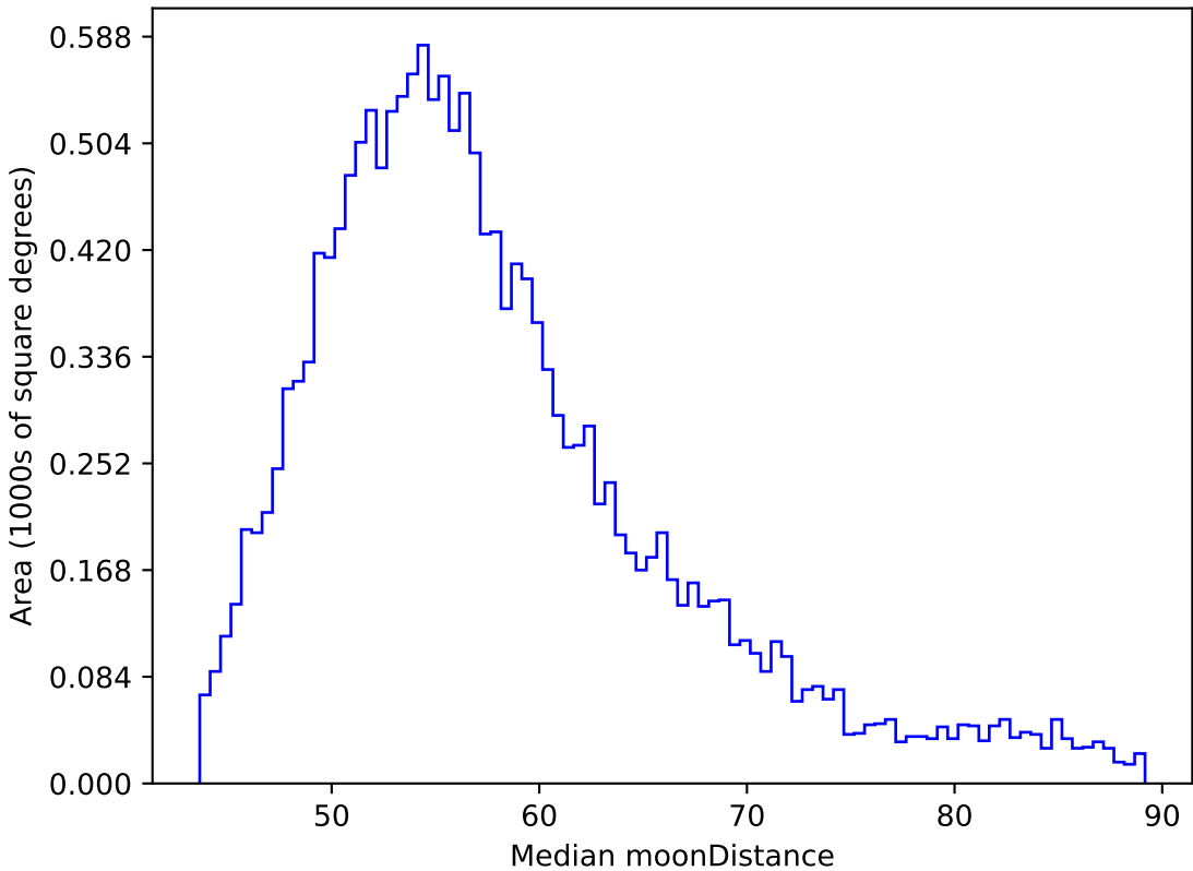
ddf_loaded_fl8_v3.4_10yrs WFD y band: Median moonDistance
